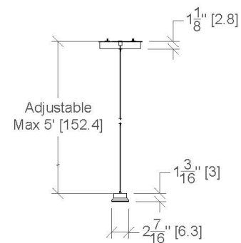
RIGHT VIEW
