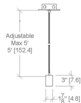
RIGHT VIEW
