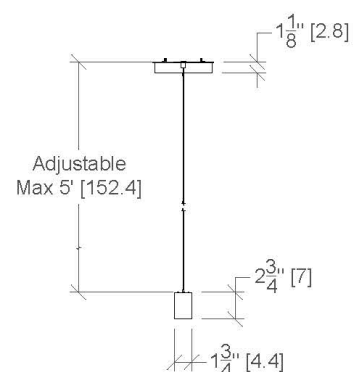
RIGHT VIEW
