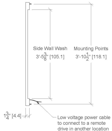
RIGHT VIEW
