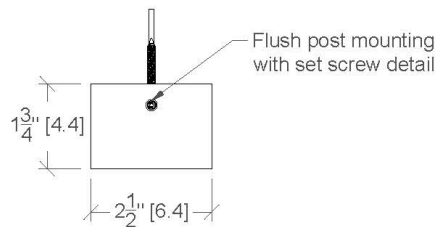
DETAIL A SCALE 1:3
