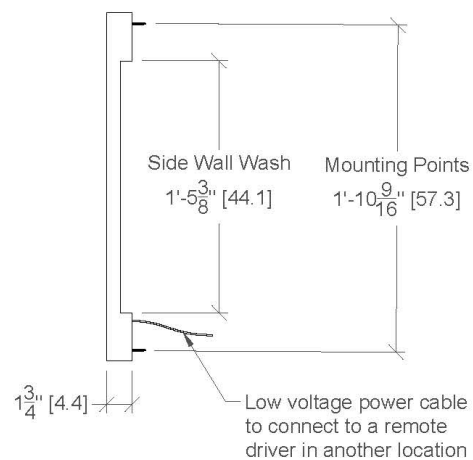
RIGHT VIEW
