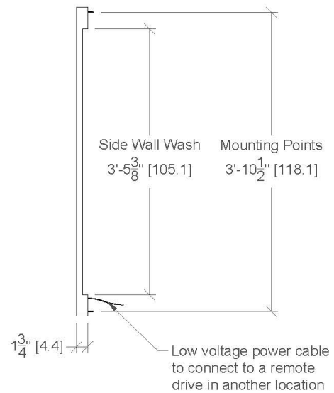
RIGHT VIEW
