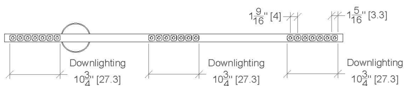
BOTTOM VIEW
